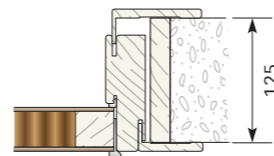
SP 125 mm - standard
