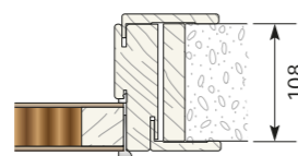
SP 108 mm - standard
